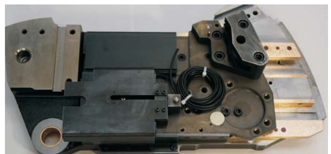
▲ Coiling plate after repair
