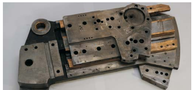
▲ Coiling plate before repair
